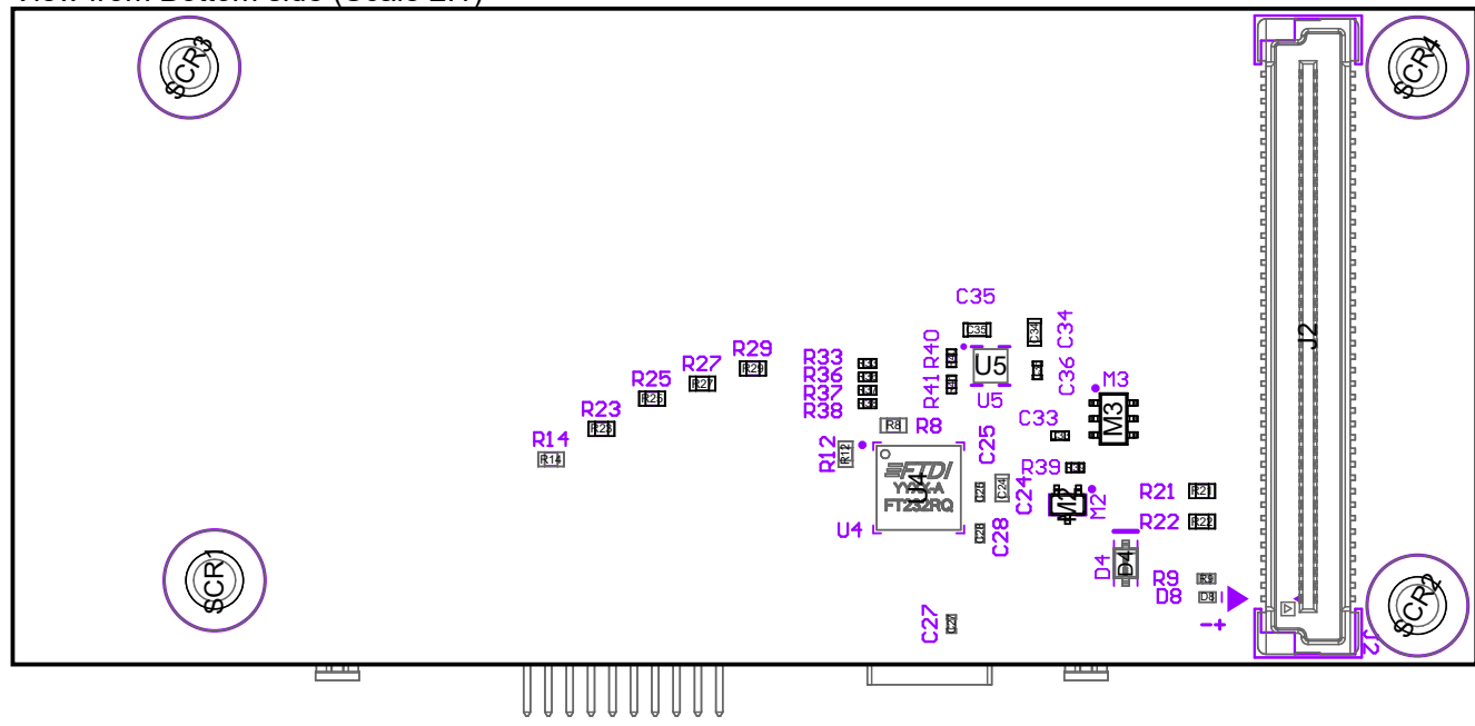
View from Bottom side (Scale 2:1)
