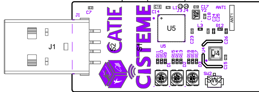
View from Top side (Scale 2:1)
