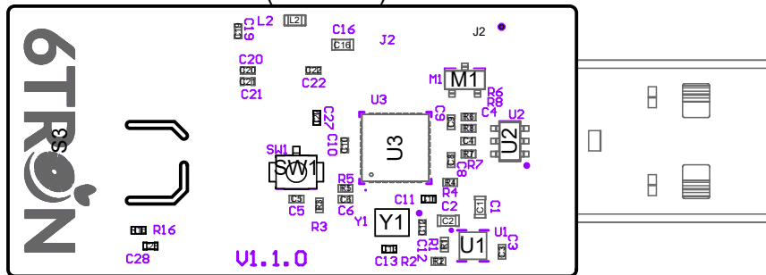
View from Bottom side (Scale 2:1)
