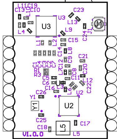
View from Top side (Scale 2:1)
